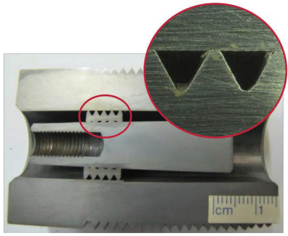
Figure 4. Pop-A-Plug sectioned serration detail.
