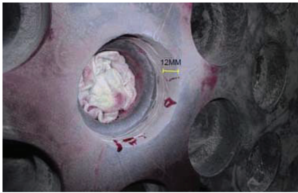
Figure 2. Significant cracking within the heat-affected zones resulting from the use of welded plugs in the waste heat boiler.
